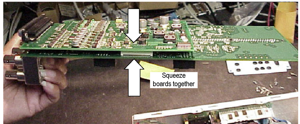
Figure 9: Checking the inter-board connection
