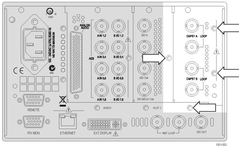
Figure 7: Removing the Option CPS rear-panel screws
