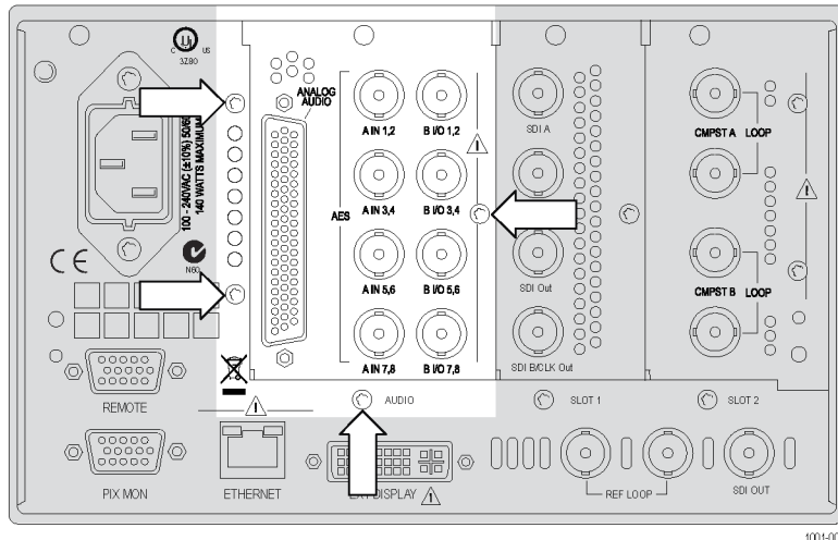
Figure 10: Removing the audio rear panel screws
